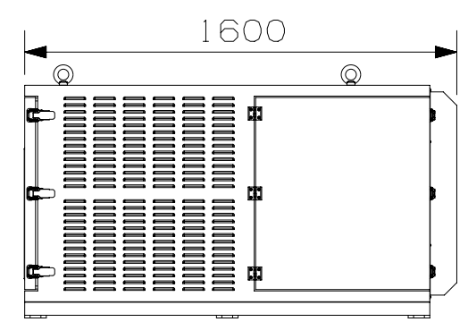
VIEW F
