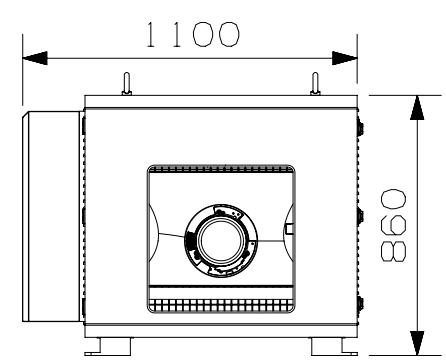
VIEW B
