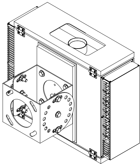
Isometric@31
