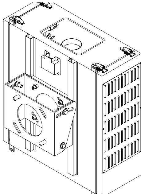
Isometric@6
